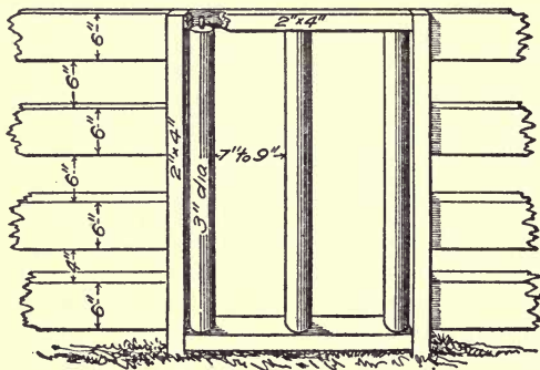
Lamb creep with rollers for uprights. (U. S. Farmers' Bul. No. 810)
