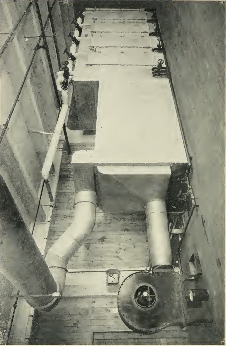
A type of tray dryer
